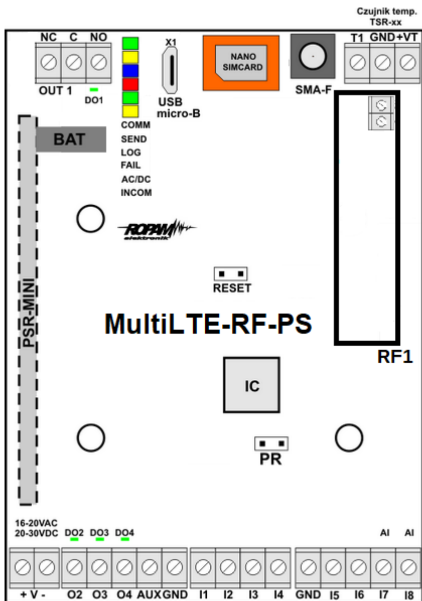
Widok MultiLTE-RF-PS.
